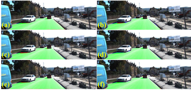
Fig. 6: An example of testing images on the KITTI road benchmark, where (a)-(f) shows the road prediction obtained by MultiNet [24], StixelNet II [25], RBNNet [26], LC-CRF [27], LidCamNet [23] and our proposed NIM-RTFNet, respectively. Correctly detected drivable areas are in green. Red pixels correspond to false negatives, whereas blue pixels denote false positives.
